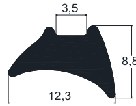
AYKİM02 CAM FITİLİ Glass Gasket
